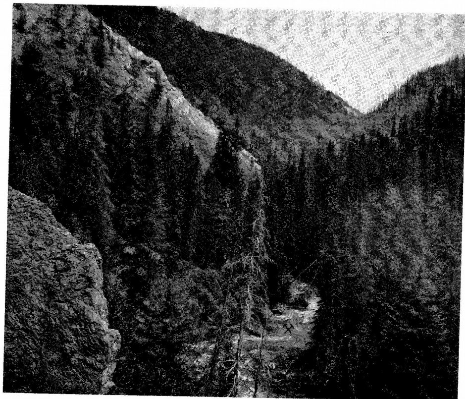
FIGURE 19. View downstream on Tyaughton Creek, Taseko Lakes area, British Columbia. The rocks are broken by many faults. The crossed hammers are positioned immediately to the right of the place where the Cassianella beds (Upper Suessi Zone) are overlain by the Marshi Zone (page 76).
