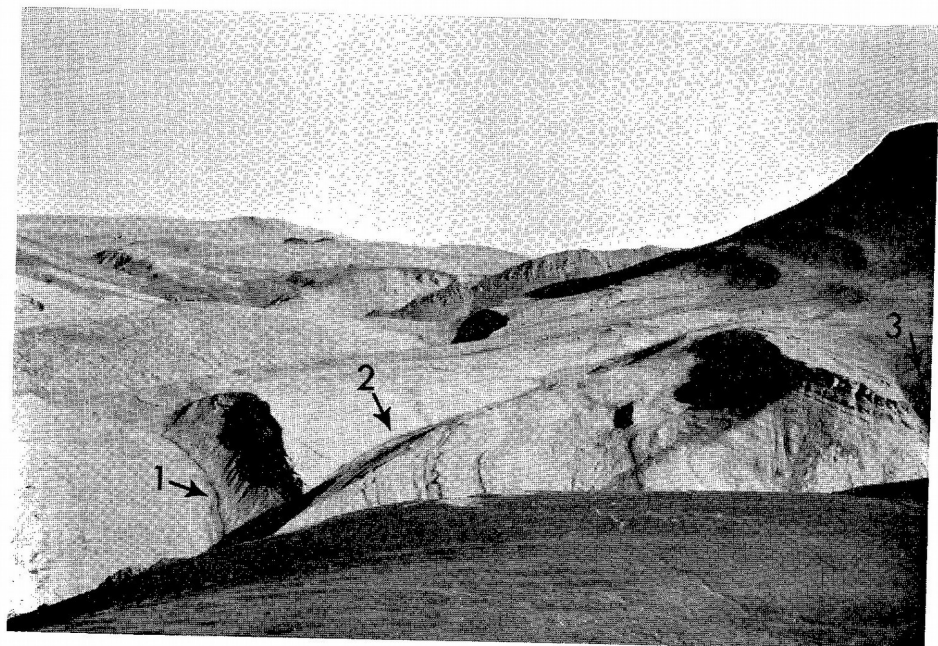
FIGURE 6. Bluffs south of Diener Creek, south of Otto Fiord, Ellesmere Island (Bukken Fiord area). (1) indicates the position of the contact between Permian rocks and the Blind Fiord Formation; Otoceras sp. occurs in the steep cutbank to the right. The Strigatus and Candidus Zones are in sequence on the slope indicated by (2). (3) shows the position of the Sverdrupi Zone.
